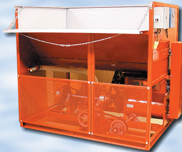
Rear detail: Airlock Exhauster
